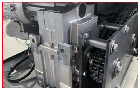
The Kobra GAMBLER is equipped with the "Titan-Colossus" gearmotor drive, specially designed heavy duty cutting knives with unmatched power to shred large quantities of casino gaming pieces such as dice, chips, gaming tokens and playing cards.
