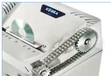
Heavy duty chain drive with steel gears.
